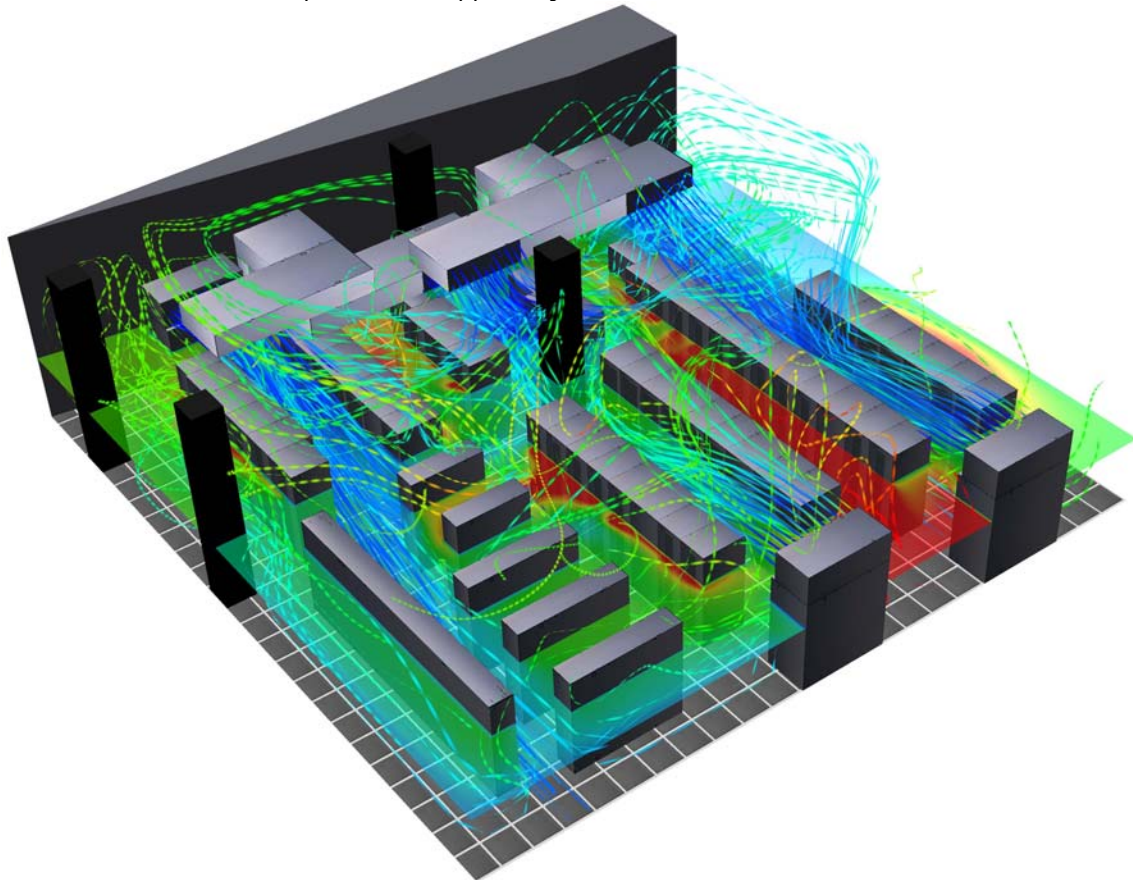
Figure 2 – 3D Computational Fluid Dynamics (CFD) model of a data center showing airflows and temperatures (supplied by APC Professional Services)
