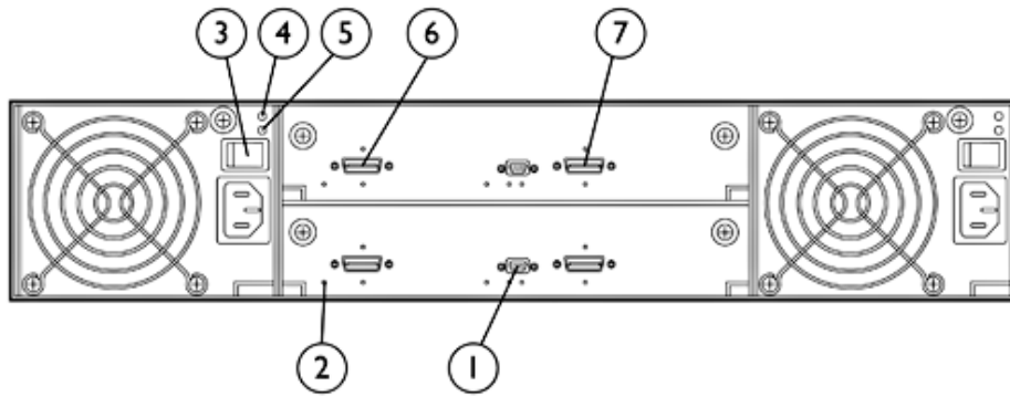
MSA2000 Dual I/O 3.5" 12 Drive Enclosure
